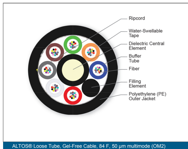
ALTOS® Loose Tube, Gel-Free Cable, 84 F, 50 µm multimode (OM2)
