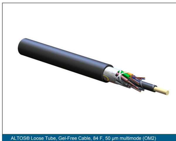
ALTOS® Loose Tube, Gel-Free Cable, 84 F, 50 µm multimode (OM2)
